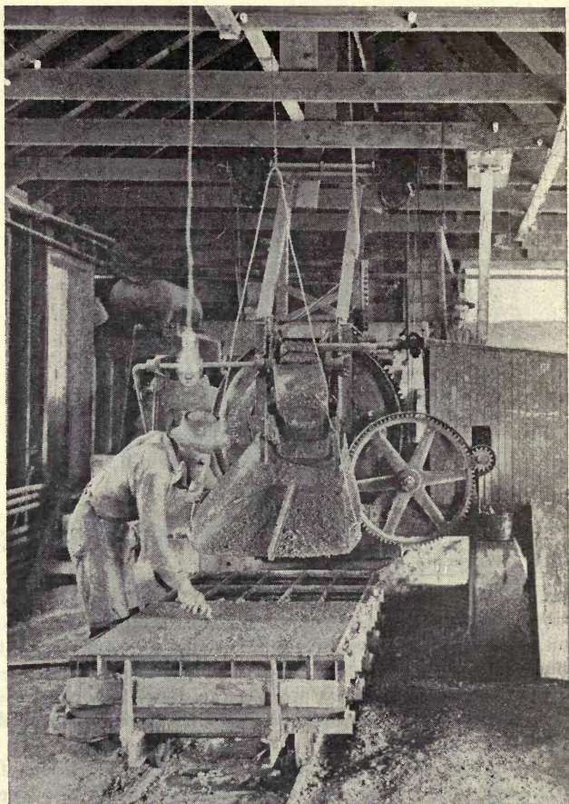
FIG. 15—GANG MOLD FOR 20 BLOCK, MOUNTED ON TRUCKS BEING FILLED WITH SLUSH CONCRETE DIRECT FROM MIXER CHUTE
